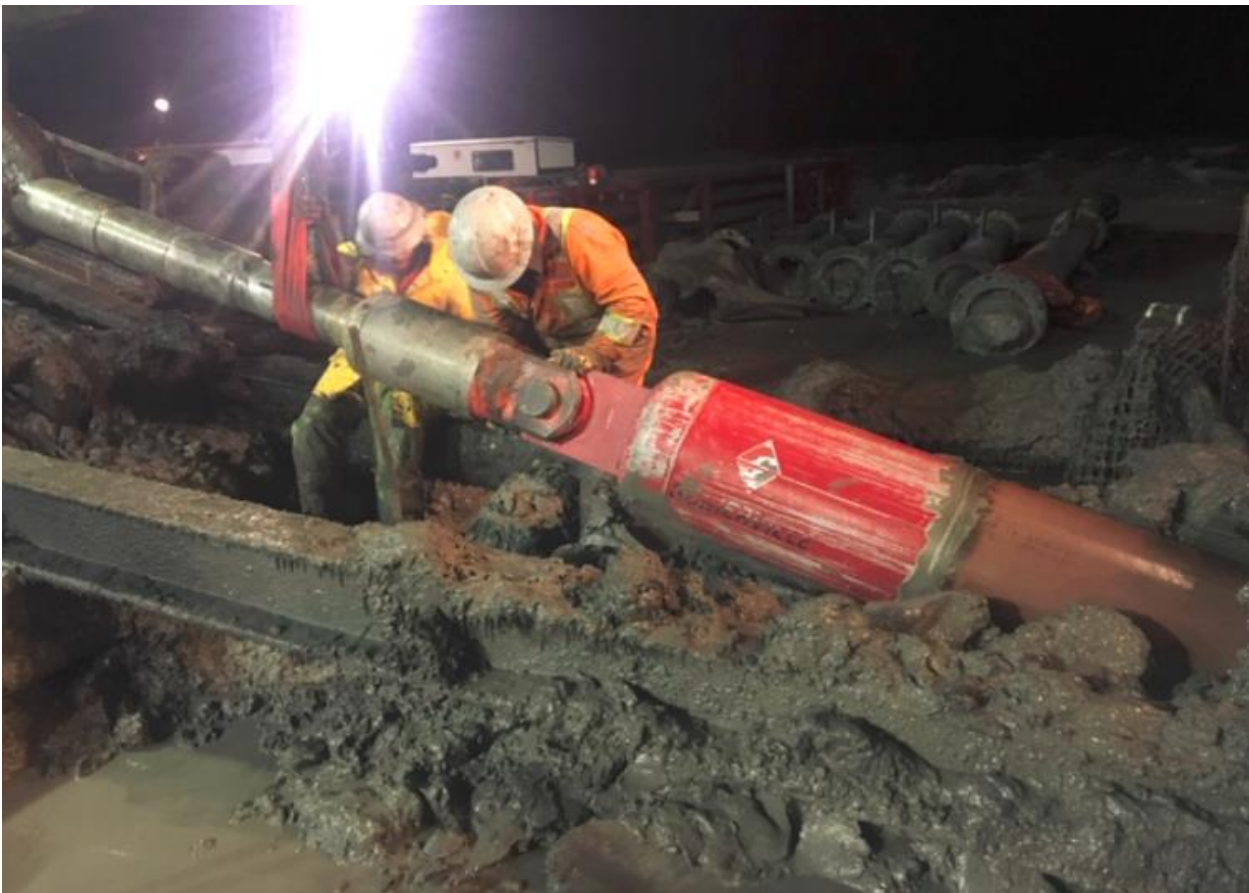
Pipe Pulled Under River: Entry Side
